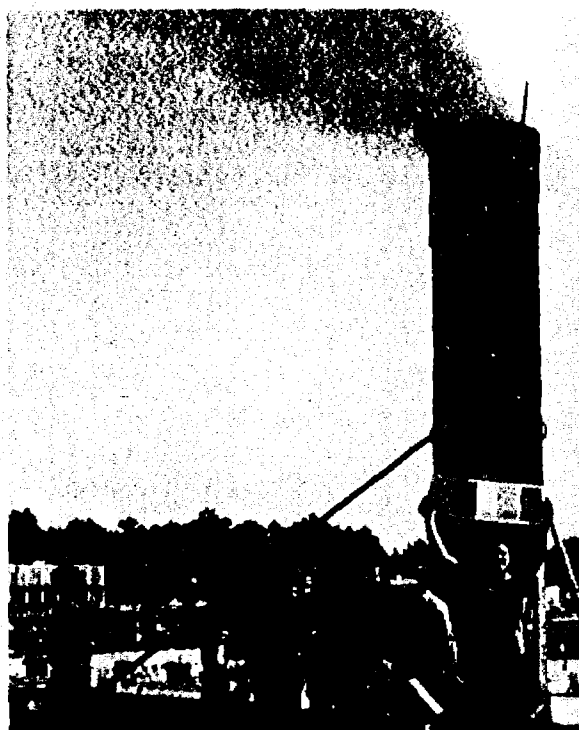
Figure 6 Use of the Ringelmann Chart for estimating emissions will probably decrease as more sophisticated sampling methods are developed.
