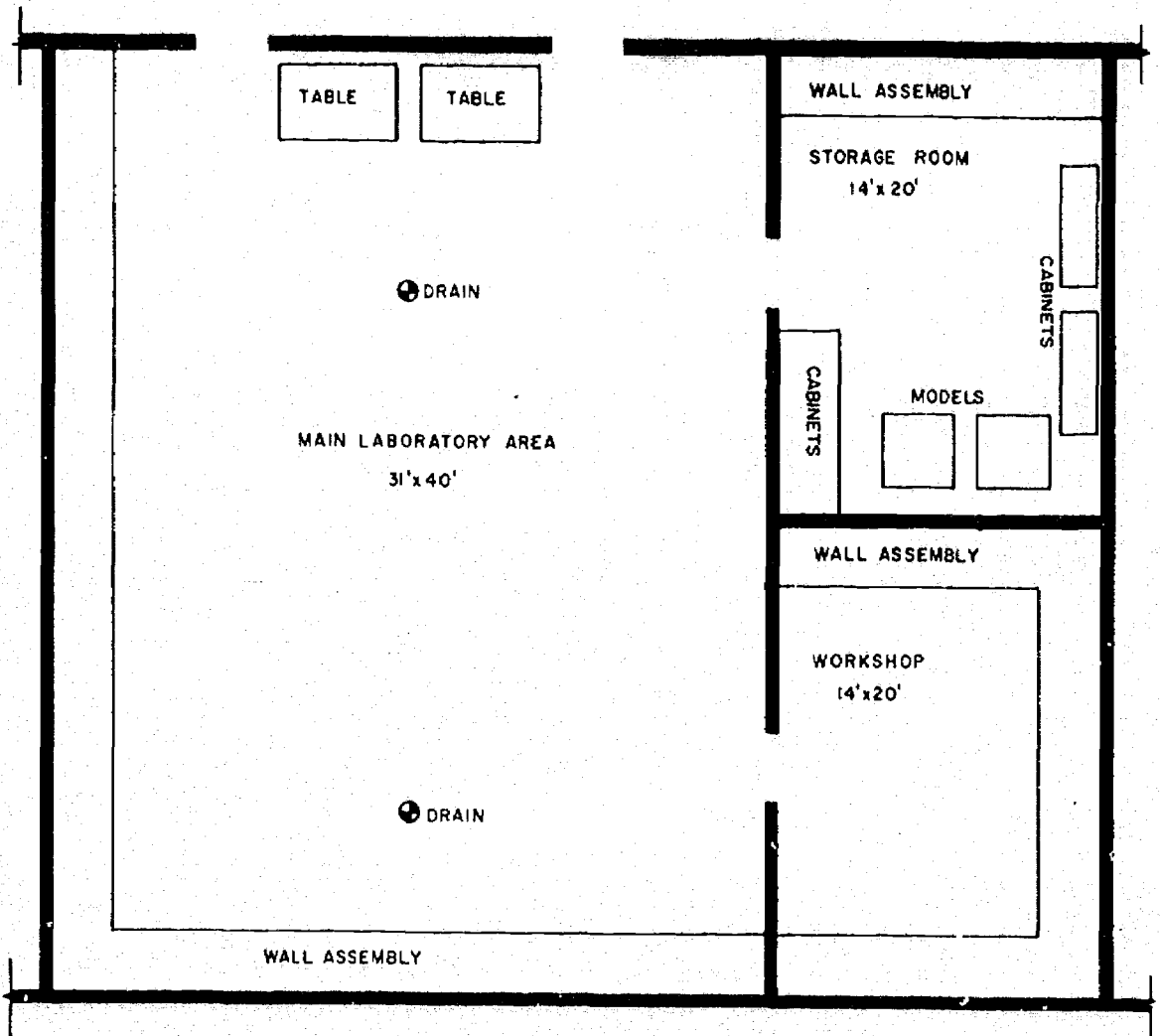
AIR POLLUTION UNIT OPERATIONS LABORATORY FIGURE 24
