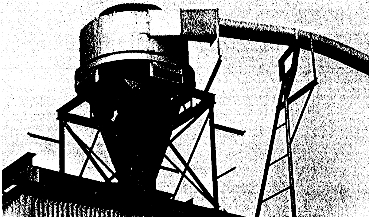
Figure 19— A simple rooftop cyclone can efficiently remove heavy particulate matter from a discharge gas stream.
